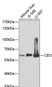
Fig. 1. Western blot analysis of extracts of various cell lines, using CES1 antibody at 1:1000 dilution. Secondary antibody: HRP-labeled Goat Anti-Rabbit IgG(H+L) (A0208) at 1:1000 dilution. Lysates/proteins: 25µg per lane. Blocking buffer: QuickBlock™ Blocking Buffer (P0231).
