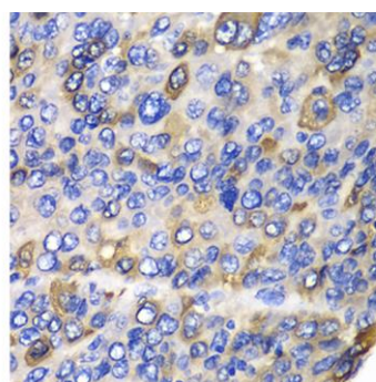
Fig. 2. Immunohistochemistry of paraffin-embedded human liver cancer using CES1 antibody at dilution of 1:100 (40x lens).
